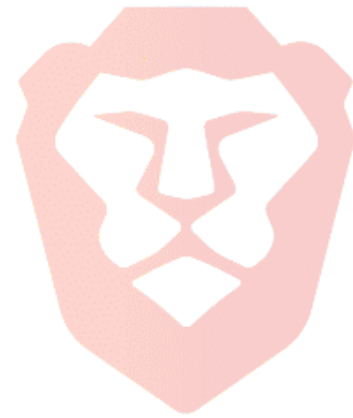
Brave
