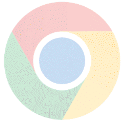
Google Chrome
