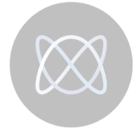
Ladybird
