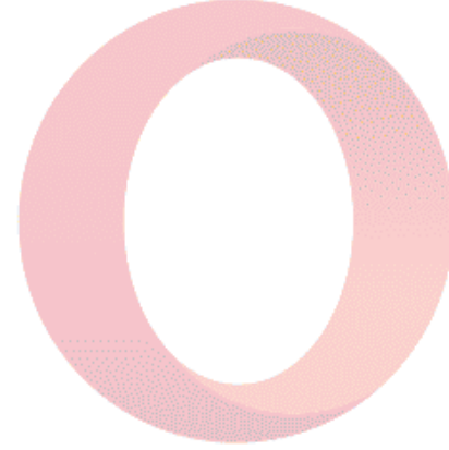
Opera
